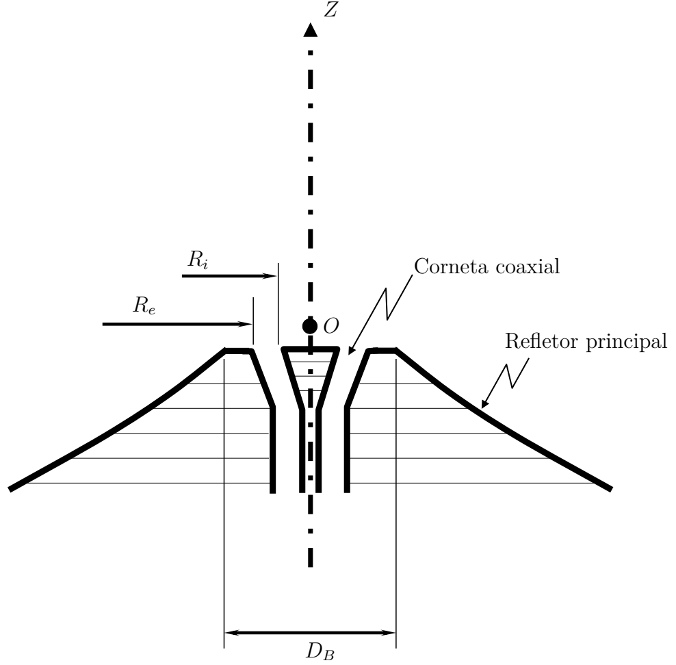
Figura 4.10 – Corneta coaxial.
