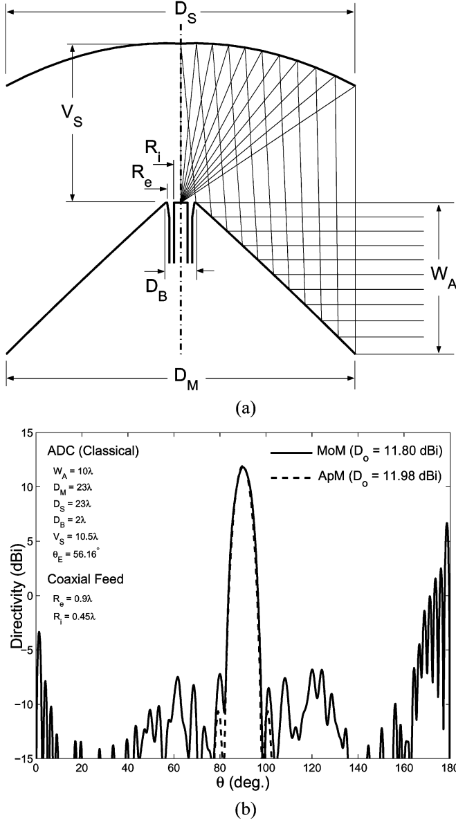
Fig. 3. Classical omnidirectional ADC antenna: (a) geometry and (b) radiation pattern.
