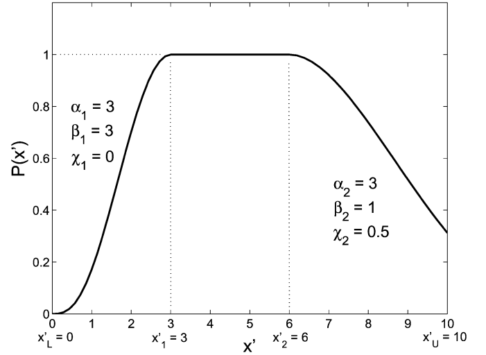
Fig. 7. Proposed tapered aperture power density.
