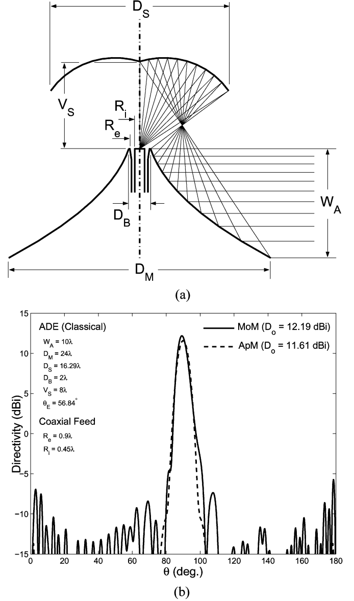
Fig. 4. Classical omnidirectional ADE antenna: (a) geometry and (b) radiation pattern.
