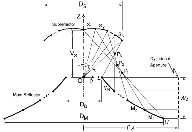
Fig. 3 Consecutive conic sections generating the omnidirectional ADE dual-reflector system
