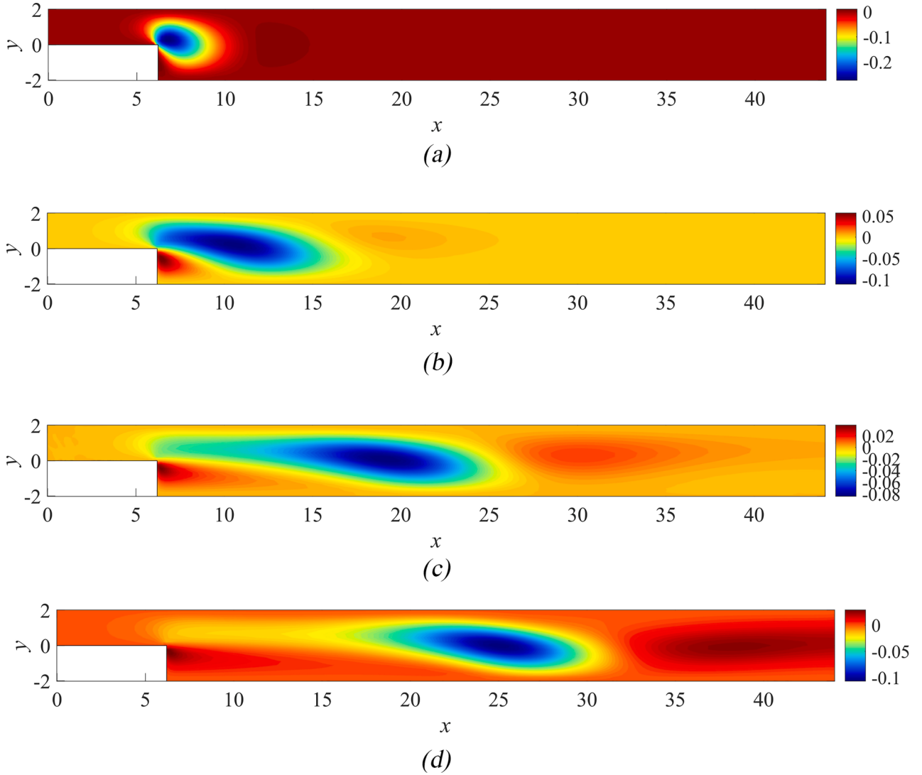
Fig. 16. The vertical component u_{h,2} provided by the \text{OFE}_1/\text{OFE}_0 pair. (a) Solution at Re = 5 . (b) Solution at Re = 50 . (c) Solution at Re = 150 . (d) Solution at Re = 250 .
