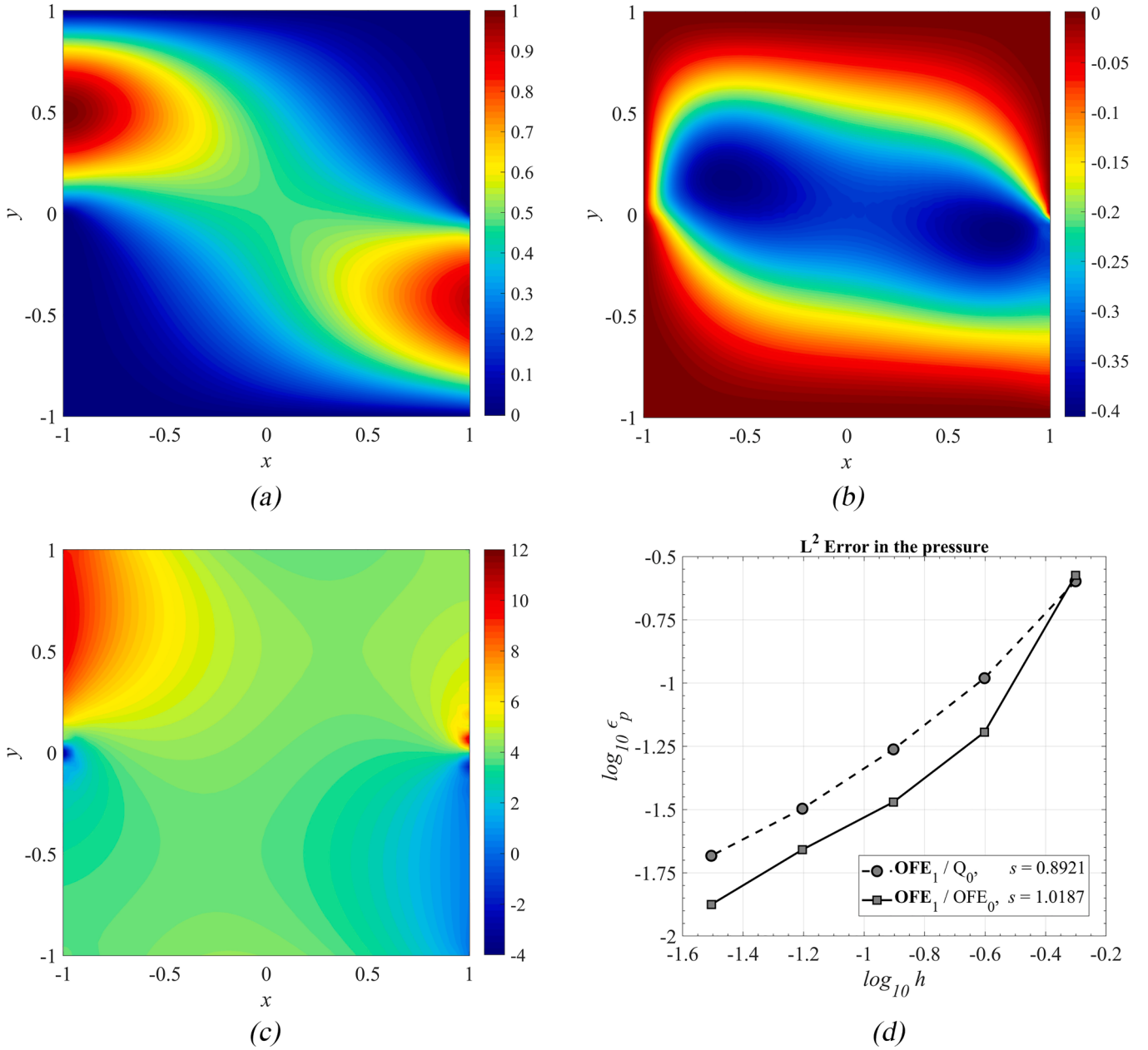
Fig. 11. Finite element solution, calculated using the \text{OFE}_1/\text{OFE}_0 pair, using a uniform mesh formed by 32 \times 32 square elements. (a) Horizontal component of the velocity field. (b) Vertical component of the velocity field. (c) The pressure field. (d) Error in the pressure for a sequence of uniform meshes ( \Delta = 0 ), using the \text{OFE}_1/Q_0 pair (black curve in Fig. 8b, shown as a dashed curve here), and using the \text{OFE}_1/\text{OFE}_0 pair (black curve in Fig. 10c). The slopes s are taken from Tables 2 and 3.
