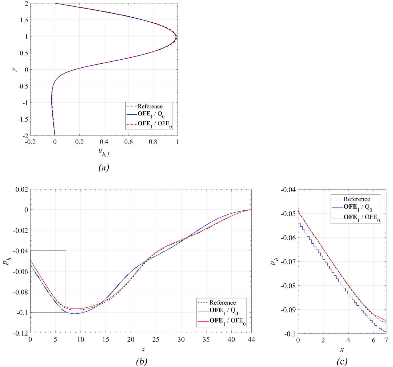
Fig. 18. Field profiles at Re = 250 , provided by the \text{OFE}_1/\mathcal{Q}_0 and \text{OFE}_1/\text{OFE}_0 pairs. (a) Horizontal component of the velocity field u_{h,1} calculated along the vertical line segment x = 7 and -2 \leq y \leq 2 (dotted orange line in Fig. 14a). (b) Pressure field p_h along the top wall (horizontal line segment 0 \leq x \leq 44 and y = 2 ). (c) Zooming in on the region marked with a rectangle in Fig. 18b. Reference solution given by the \mathcal{Q}_2/\mathcal{Q}_1 pair, using the mesh of cells in Fig. 14b. (For interpretation of the references to colour in this figure legend, the reader is referred to the web version of this article.)
