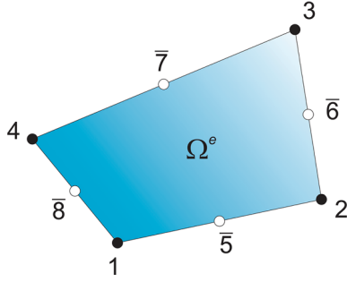
Fig. 2. A cell \Omega^e , indexed by the number 'e'. The nodes at the four vertices are indicated by the (local) indices 1, 2, 3, and 4. The DoF's (coefficients \tilde{s}_{I,m} in the expansion (3b)) are assigned to these nodes only. The points 5, 6, 7, and 8 are located at the midpoints of the edges; there are no DoF's assigned to them, since they are used just as an aid to construct the serendipity shape functions \hat{h}_{JI} in (3e), see [36].
