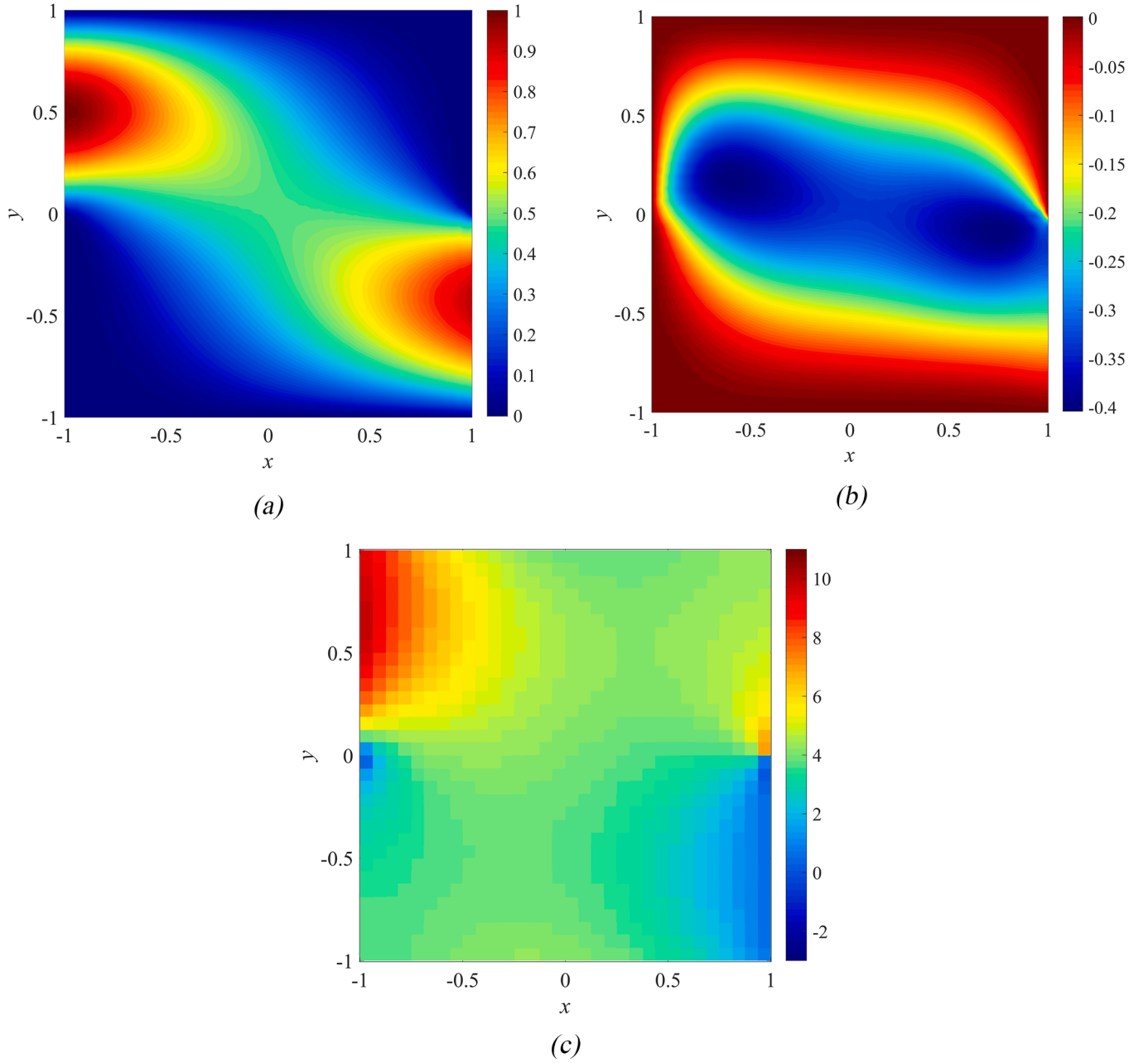
Fig. 6. Finite element solution, calculated using the \mathbf{OFE}_1/Q_0 pair, on a uniform mesh formed by 32 \times 32 square elements. (a) Horizontal component of the velocity field. (b) Vertical component of the velocity field. (c) The pressure field, this time not contaminated by the checkerboard pattern.
