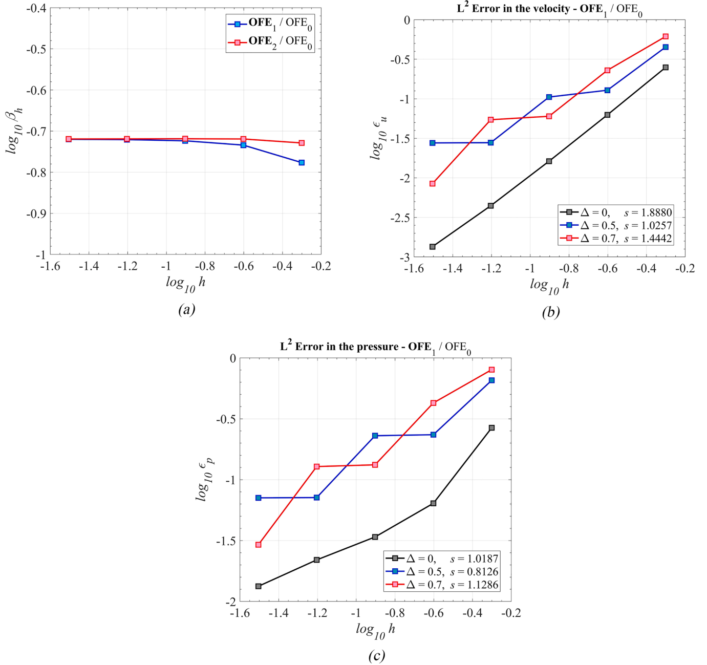
Fig. 10. (a) The inf-sup curves calculated in a sequence of uniform meshes with N \times N square elements each. Results concerning the \text{OFE}_1 / \text{OFE}_0 and \text{OFE}_2 / \text{OFE}_0 pairs, see Sections 4.2 and 4.3, respectively. For both cases, the inf-sup constants stabilize at a positive value and do not decay as h decreases. (b) Convergence curves for the velocity, using the \text{OFE}_1 / \text{OFE}_0 pair. The errors are calculated with respect to the \mathcal{Q}_2 / \mathcal{Q}_1 reference solution from Fig. 4, using (4c). (c) Convergence curves for the pressure. The approximate slopes s are taken from Table 3, and \Delta is the mesh distortion parameter.
